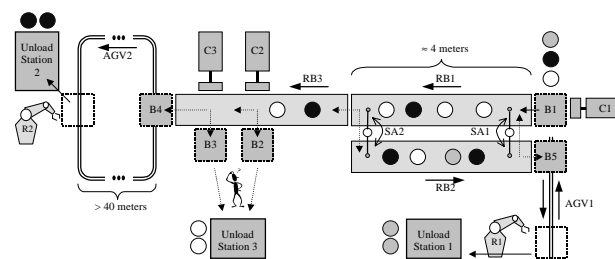
Fig. 2. Mechanical system layout
