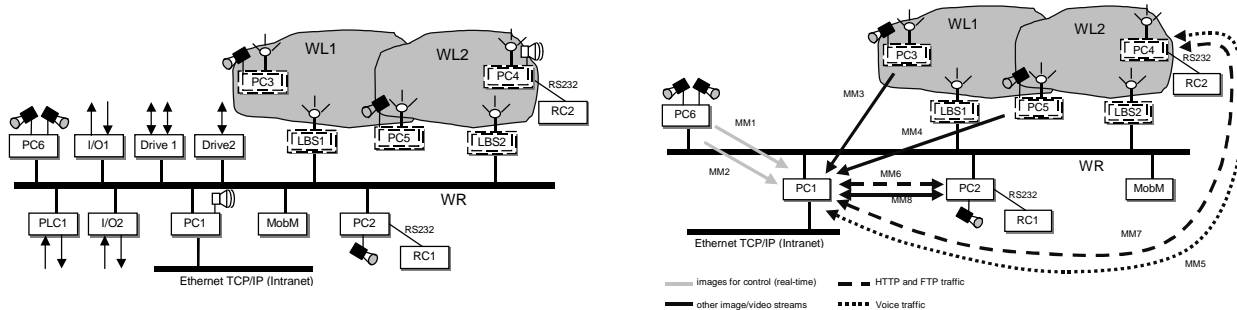
Fig. 3. RFieldbus network topology (left), Multimedia streams (right)
