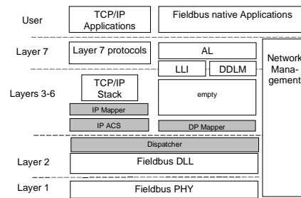
Fig. 1. PROFIBUS and TCP/IP integration
