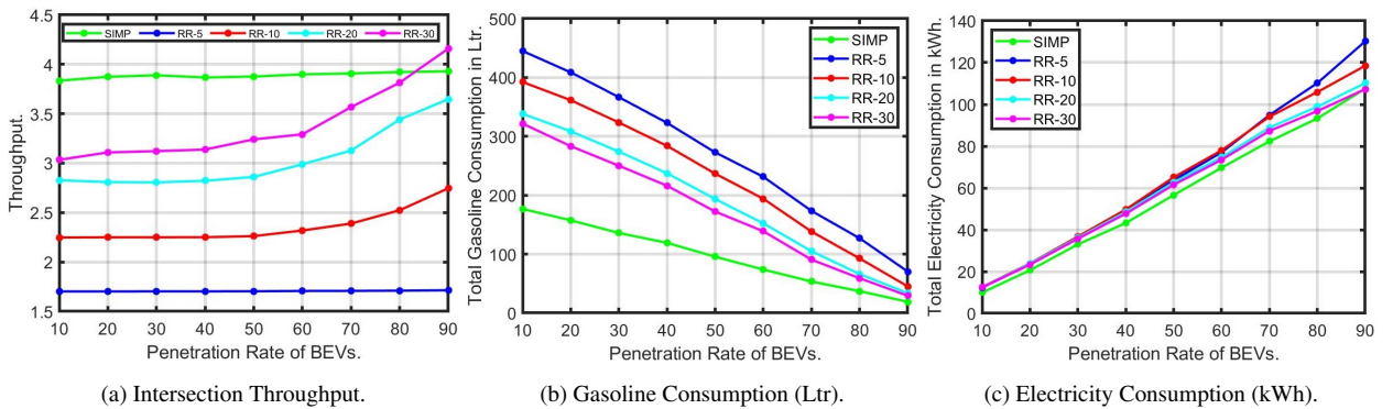
Fig. 1: Throughput, Gasoline and Electricity Consumption against Battery Electric Vehicles Penetration Rate.
