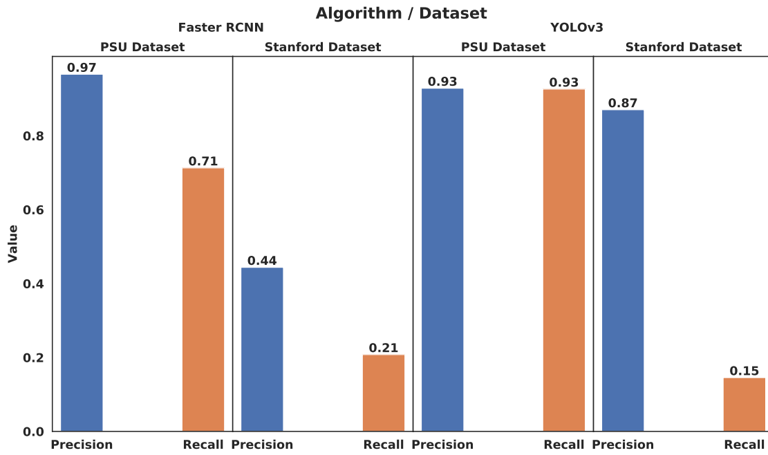
Fig. 10: Precision and recall values for YOLOv3 and Faster R-CNN, on the two datasets.
