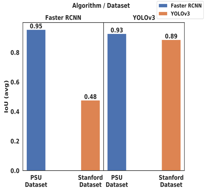
Fig. 18: Average IoU value for YOLOv3 and Faster R-CNN, on the two datasets.
