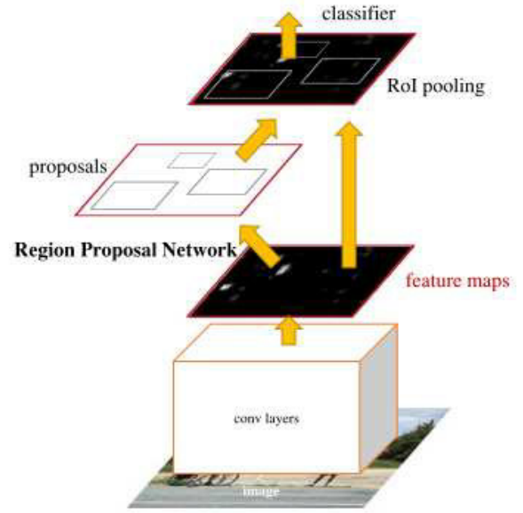
Fig. 1: Faster R-CNN basic architecture.
