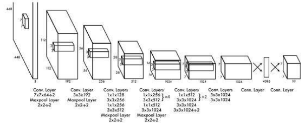
Fig. 3: YOLO (version 1) network architecture.
