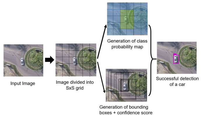
Fig. 5: Successive stages of the YOLOv3 model applied on car detection.
