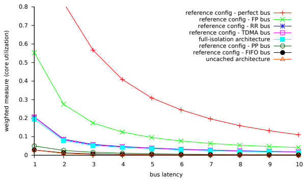
Figure 6: Weighted schedulability; varying bus latency (in cycles).
