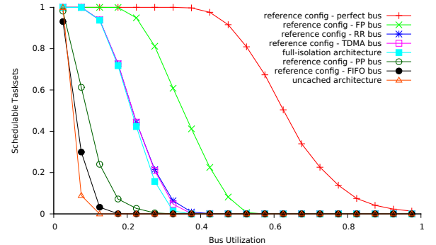
Figure 5: Number of schedulable task sets vs. bus utilization
