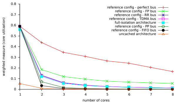
Figure 7: Weighted schedulability; varying number of cores.
