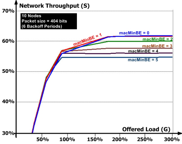
Fig. 13. The network throughput as a function of the offered load for different macMinBE values with 10 Nodes
