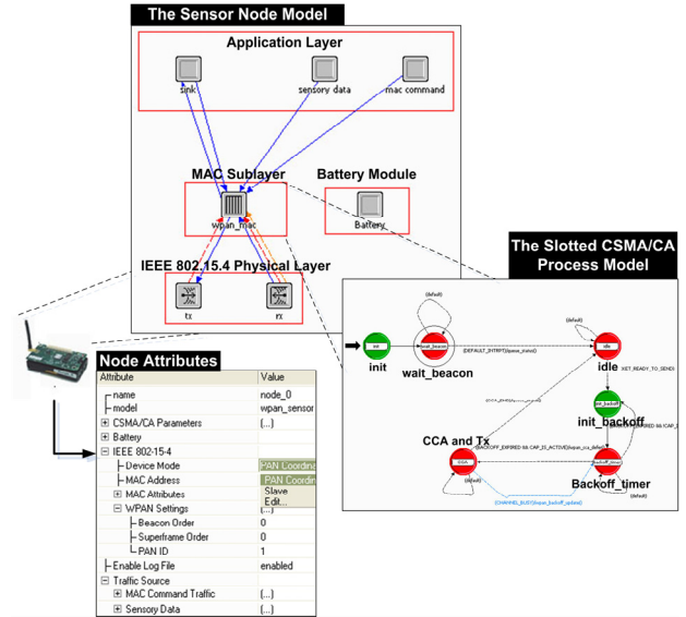
Fig. 3. Simulation model of an IEEE 802.15.4 sensor node
