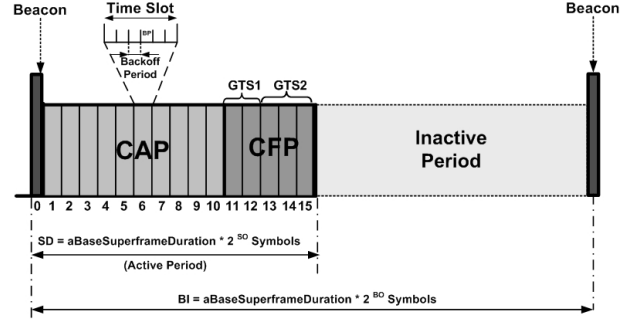
Fig. 1. Beacon interval and superframe concepts
