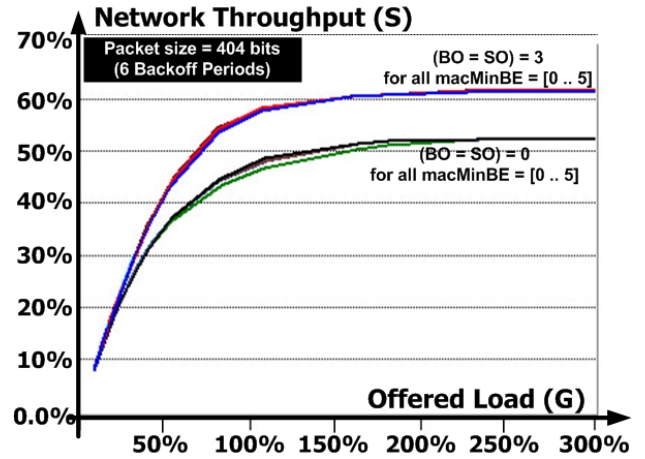
Fig. 11. The network throughput as a function of the offered load for different macMinBE values
